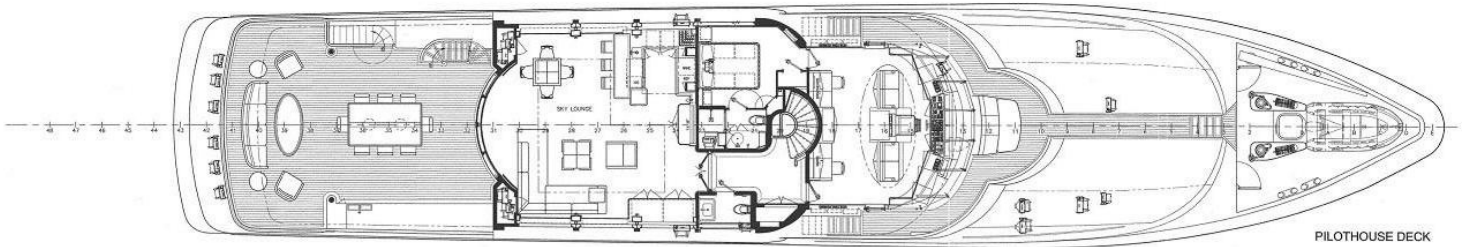
PILOTHOUSE DECK
